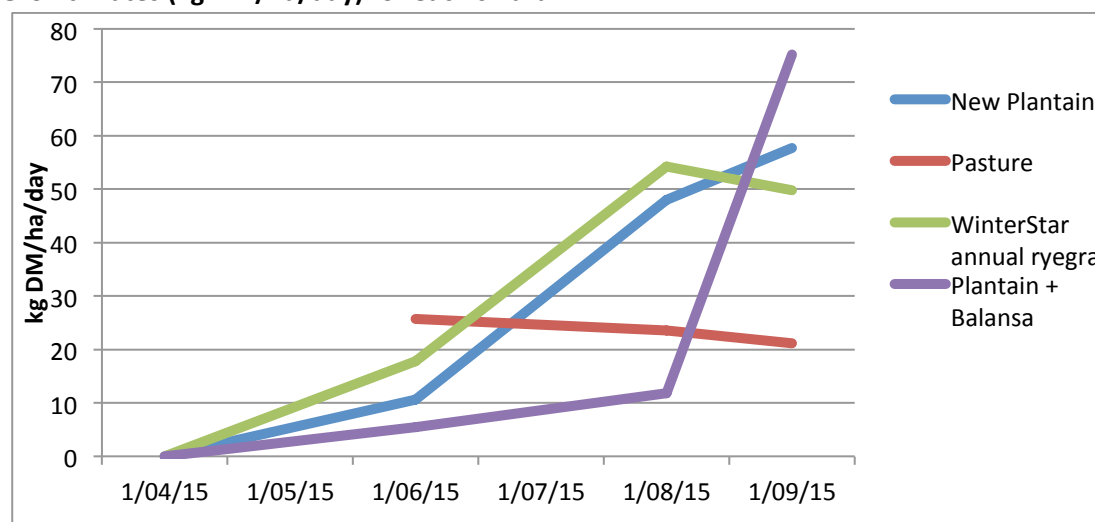
Growth rates (kg DM/ha/day) for each sward
